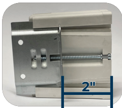
0"-2" of Adjustability
