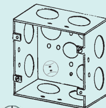
4SJD-1 2-1/8" Deep, Welded
