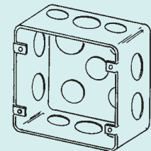
4SPJD Plenum Box 2-1/8" Deep, Drawn (Screws supplied with cover, catalog number 8487P)
