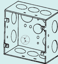
4SJD-3/4 2-1/8" Deep, Welded
