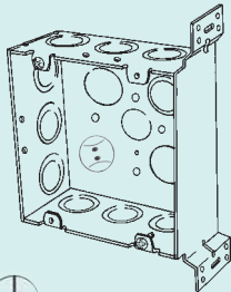
4SJD-EK-VB 2-1/8" Deep, Welded Offset vertical bracket flush with front of box
