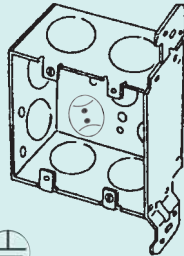
4SJD-1-VB 2-1/8" Deep, Welded Offset vertical bracket flush with front of box
