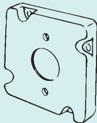
8496 1/2" Raised 1-19/32" Opening
