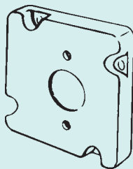
8494 1/2" Raised 1-13/32" Opening
