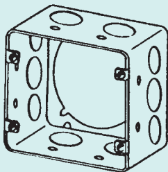
4SJDE-1/2-3/4 2-1/8" Deep, Drawn 8-32 tapped holes and slide-on screw slots in bottom
