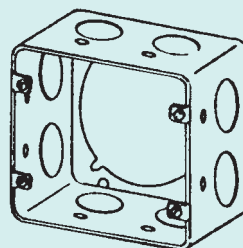
4SJDE-1 2-1/8" Deep, Drawn 8-32 tapped holes and slide-on screw slots in bottom
