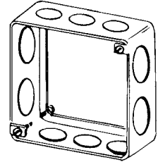
4SES Combo Extension-Thru-Ring 1/2" Deep, Drawn Top: Two 8-32 screws Bottom: Two 8-32 screws and two slide-on slots
