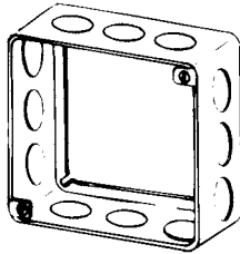
4SE-1/2 Extension Ring 1/2" Deep, Drawn Top: Two 8-32 screws Bottom: Two slide-on slots
