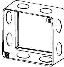
4SE-3/4 Extension Ring 1/2" Deep, Drawn Top: Two 8-32 screws Bottom: Two slide-on slots
