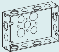
2G5075S Two Gang 6 13 / 16 " Wide, Welded
