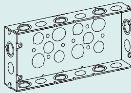
4G5075S Four Gang 10 9 / 16 " Wide, Welded
