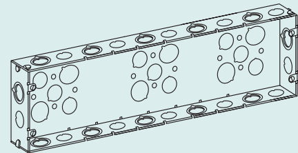
8G5075S Eight Gang 17 3 / 4 " Wide, Welded
