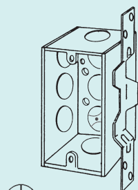
4SSLVB-1/2 2-1/8" Deep, Welded Plain vertical bracket set back 3/4"
