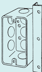
4CSL-1/2 1-1/4" Deep, Drawn
