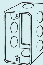
4SSLE-1/2 1-1/2" Deep, Drawn
