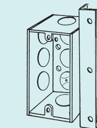
4SSLX-1/2PL 2-1/8" Deep, Welded Plain vertical angle bracket set back 5/8"
