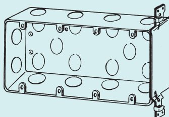
134APFB-1/2 2-1/2" Deep, Welded Four Gang – 7-1/2" Wide Stud NL bracket set back 1/2"
