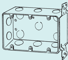
133APFB-1/2 2-1/2" Deep, Welded Three Gang – 5-3/4" Wide Plain offset side combination bracket set back 1/2"
