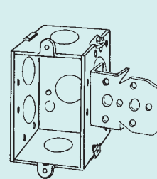
222NL 2-1/2" Deep, Gangable Stud NL bracket set back 1/2"
