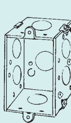
222LE 2-1/2" Deep, Gangable Four nail holes each side side leveling bosses
