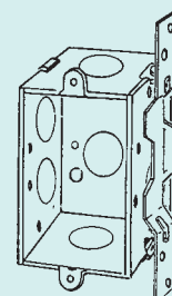
222VB-PL 2-1/2" Deep, Gangable Plain vertical bracket set back 3/4"
