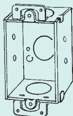
94 1-1/2" Deep, Welded Plaster ears*
