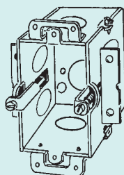
222-OW 2-1/2" Deep, Gangable Old work-support clamps Plaster ears*
