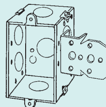
222NL 2-1/2" Deep, Gangable Stud NL bracket set back 1/2"
