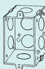
111LE 2" Deep, Gangable Four nail holes each side side leveling bosses
