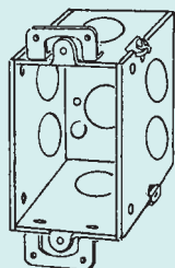
333 2-3/4" Deep, Gang- able Plaster ears*
