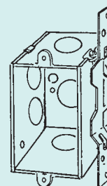
333VB 2-3/4" Deep, Gangable Plain vertical bracket set back 3/4"
