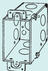
333D 3-1/2" Deep, Gangable Plaster ears*
