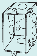
333LE 2-3/4" Deep, Gangable Two nail holes each side side leveling bosses
