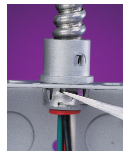
To remove from box, lift Snap-Tite ® ring with a screwdriver and twist off.
