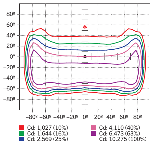
ISOCANDELA PLOT
