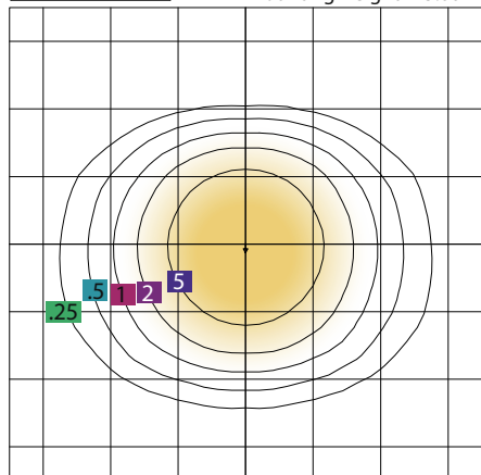
PHOTOMETRY FLL340-150W-WIDE BEAM Mounting Height=15.00 FT
