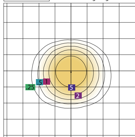
PHOTOMETRY FLL330-100W-WIDE BEAM Mounting Height=15.00 FT
