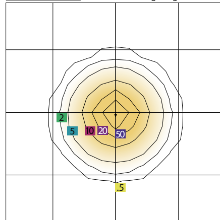
PHOTOMETRY FLL350-300W-3 X 3 Mounting Height=30.00 FT
