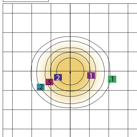
PHOTOMETRY FLL310-20W-WIDE BEAM MOUNTING HEIGHT=15.00 FT
