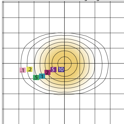
PHOTOMETRY FLL350-300W-WIDE BEAM Mounting Height=30.00 FT
