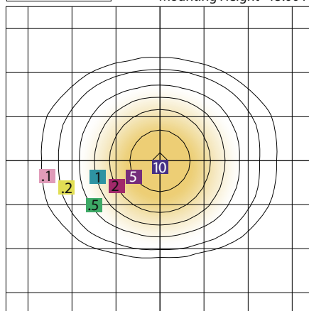
PHOTOMETRY FLL320-50W-WIDE BEAM Mounting Height=15.00 FT
