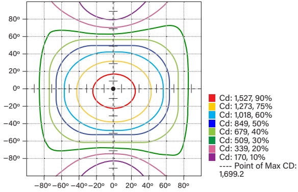
ISOCANDELA PLOT
