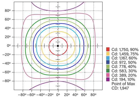
ISOCANDELA PLOT
