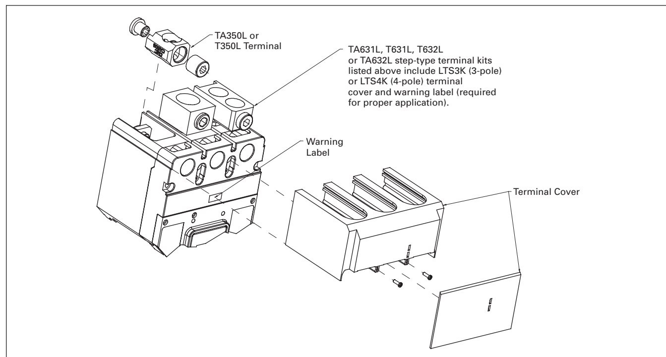
Figure 1. Terminals and Terminal Cover for the LG Breaker — Includes LTS3K (3-Pole) or LTS4K (4-Pole) Terminal Covers
