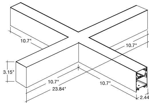
LED-ALIN2-FL-22X22-X-3P50-D-5CCT-WH
