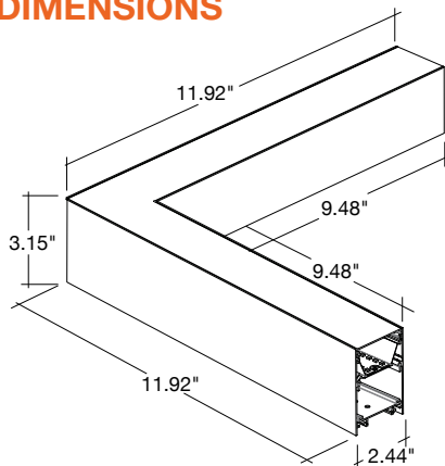
LED-ALIN2-FL-12X12-L-3P25-D-5CCT-WH
