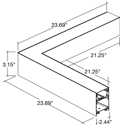
LED-ALIN2-FL-24X24-L-3P50-D-5CCT-WH
