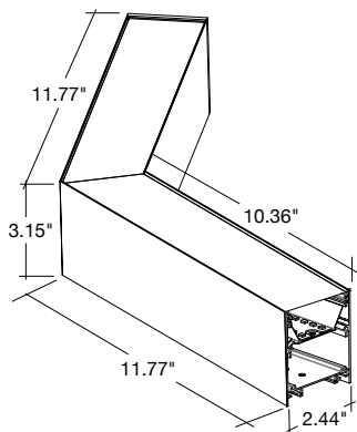
LED-ALIN2-FL-12X12-135L-3P25-D-5CCT-WH
