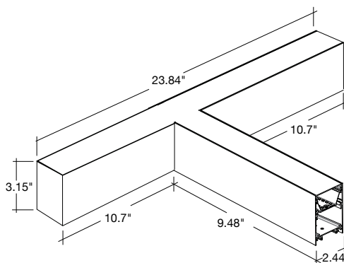
LED-ALIN2-FL-22X10-T-3P50-D-5CCT-WH
