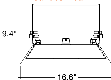
Surface Mount
