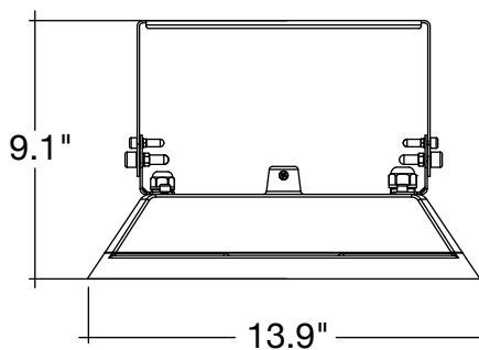
Surface Mount
