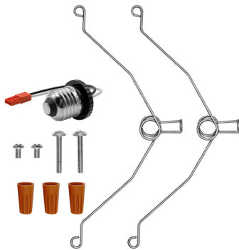
CDSK-6-CLIP
