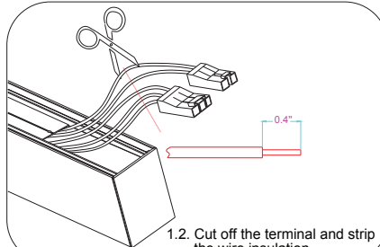
1.2. Cut off the terminal and strip the wire insulation
