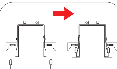
1.7. Secure to the ceiling grid (T-grid)
