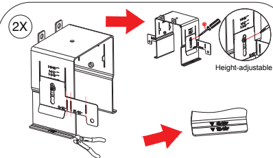
1.4. Use pliers to bend and adjust the brackets 9/19 & 15/16 according to the actual bracket width and adjust the bracket height
