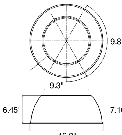
Aluminum Reflector
