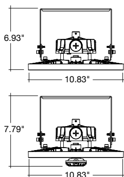
Surface Mount
