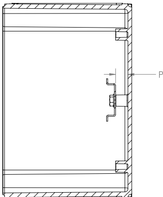
(BASE SIDE SECTION VIEW WITH DIN RAIL)
