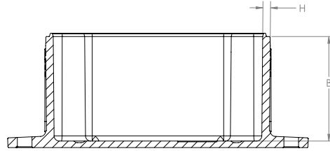
(BASE SIDE SECTION VIEW)
