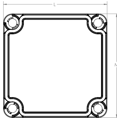
(LID BOTTOM VIEW)
