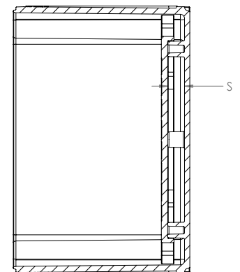
(BASE SIDE SECTION VIEW WITH BACKERPLATE)
