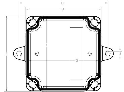
(BASE TOP VIEW)
