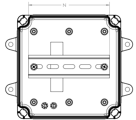
(BASE TOP VIEW WITH DIN RAIL)
