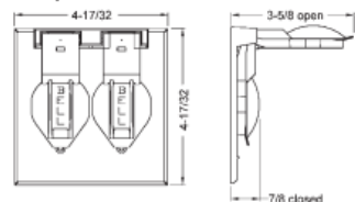
TWO-GANG DEVICE COVERS 5148-0 SERIES, 5096-0, 5160-0, 5098-0
