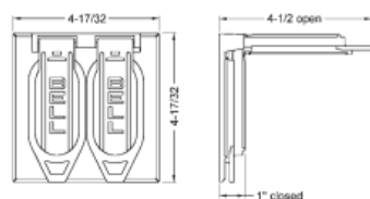
TWO-GANG DEVICE COVERS 5148-0 SERIES, 5096-0, 5160-0, 5098-0
