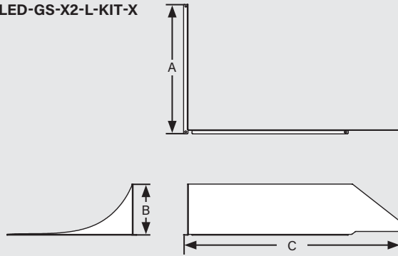
KT-ALED-GS-X2-L-KIT-X
