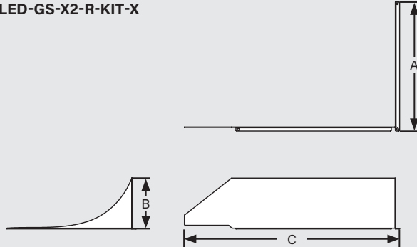
KT-ALED-GS-X2-R-KIT-X
