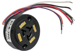
Twist-lock Receptacle KT-RSC-7PN
