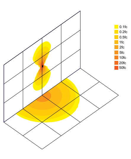
KT-CYLED10PS-3A-WDI-OSG-8CSB-VDIM (15FT MOUNTING HEIGHT, 60°)
