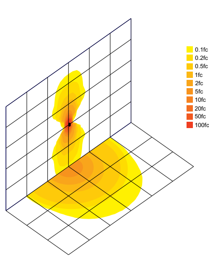
KT-CYLED36PS-6A-WDI-OSG-8CSB-VDIM (20FT MOUNTING HEIGHT, 40°)
