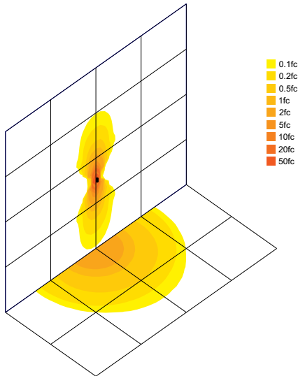
KT-CYLED10PS-3A-WDI-OSG-8CSB-VDIM (15FT MOUNTING HEIGHT, 40°)
