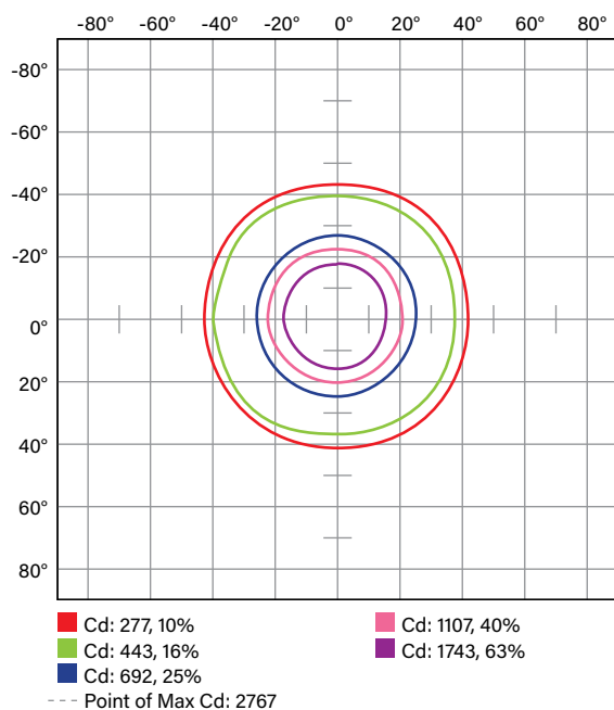
ISOCANDELA PLOT
