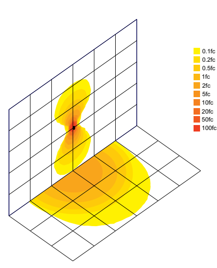
KT-CYLED36PS-6A-WDI-OSG-8CSB-VDIM (20FT MOUNTING HEIGHT, 60°)
