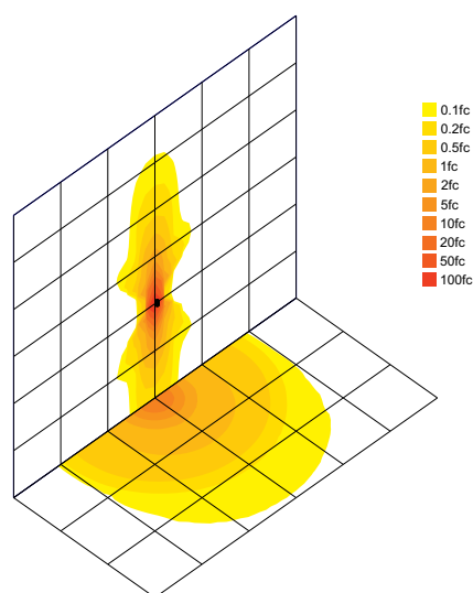
KT-CYLED36PS-6A-WDI-OSG-8CSB-VDIM (20FT MOUNTING HEIGHT, 25°)
