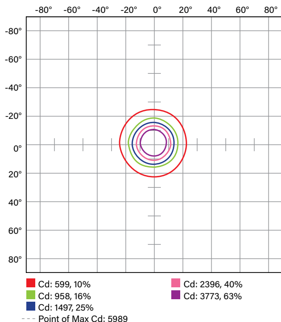
ISOCANDELA PLOT
