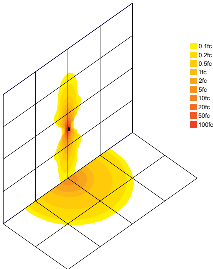
KT-CYLED10PS-3A-WDI-OSG-8CSB-VDIM (15FT MOUNTING HEIGHT, 25°)
