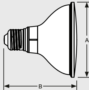
KT-LED10PAR30S-F-9CSF /G4 KT-LED10PAR30S-NF-9CSF /G4
