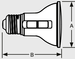
KT-LED5.5PAR20-F-9CSF /G4 KT-LED6.5PAR20-F-8CSF /G4
