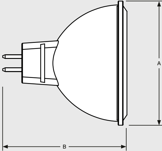
KT-LED7MR16-S-8XX /G4
