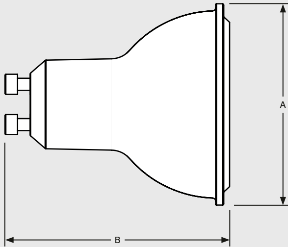
KT-LED7MR16-S-8XX-GU10 /G4
