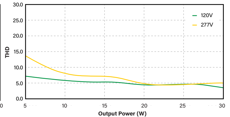
THD vs OUTPUT POWER
