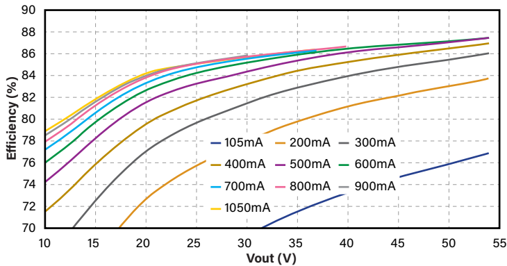
EFFICIENCY (120V)
