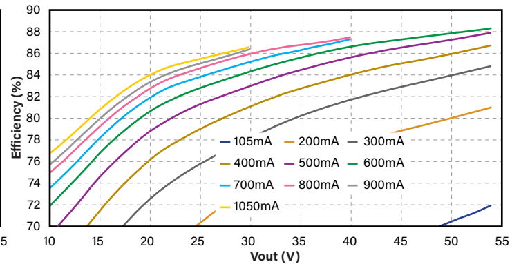
EFFICIENCY (277V)
