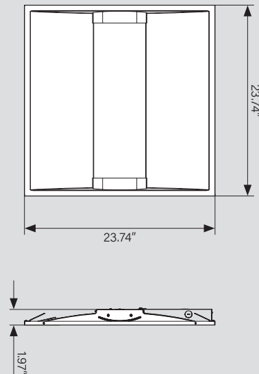
KT-RKIT24PS-22DC-8CSA-VDIM /CR KT-RKIT35PS-22DC-8CSA-VDIM /CR
