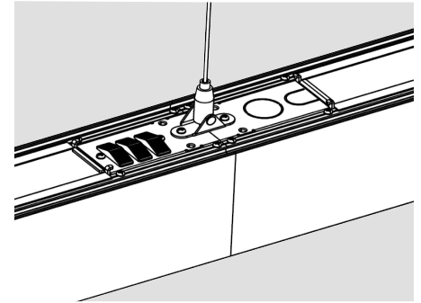
Step 3. Install suitable suspension hardware ((1) fixed aircraft cable gripper bridged across the fixture seam is recommended)
