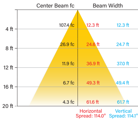
ILLUMINANCE AT A DISTANCE
