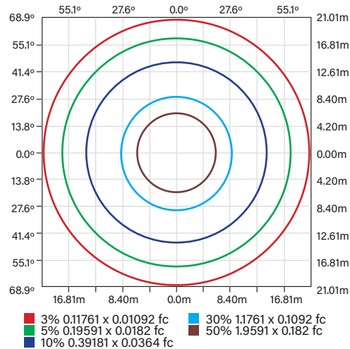
ISOCANDELA PLOT
