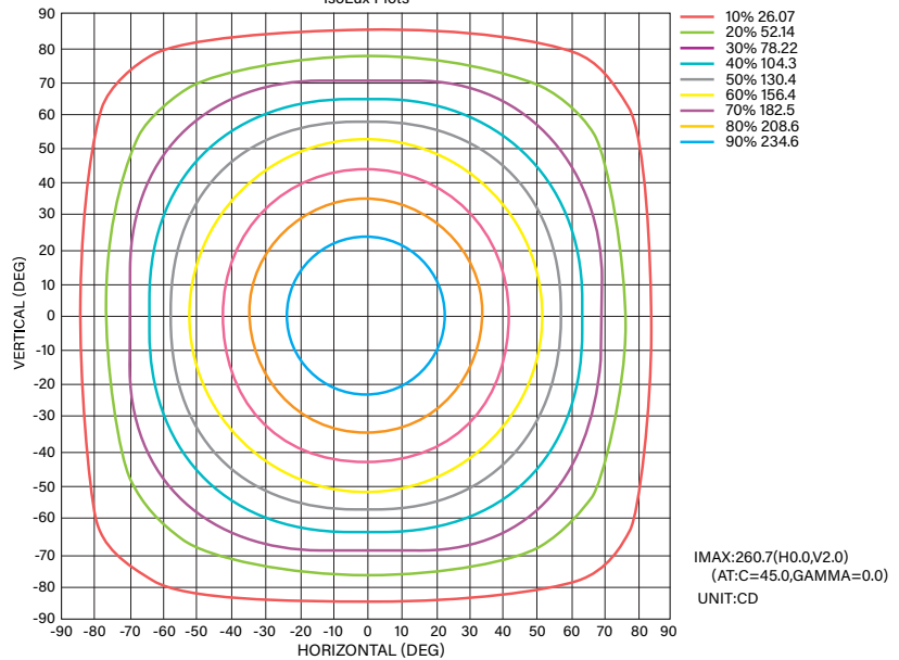
IsoLux Plots
