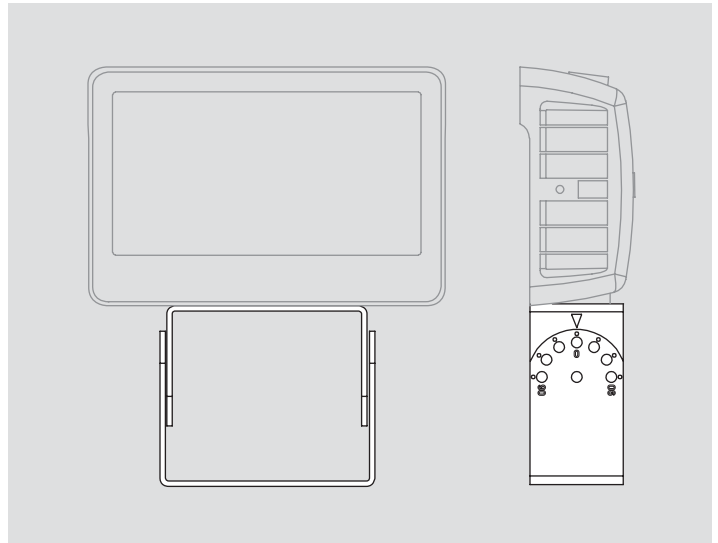
TRUNNION MOUNT (75W; 100W flood light models)
