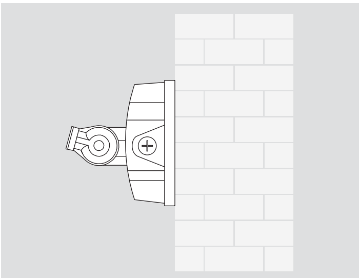
SURFACE / WALL MOUNT BOX (15W; 35W; 60W flood light models)
