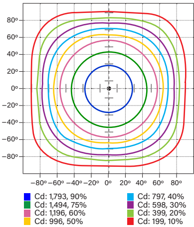
ISOCANDELA PLOT
