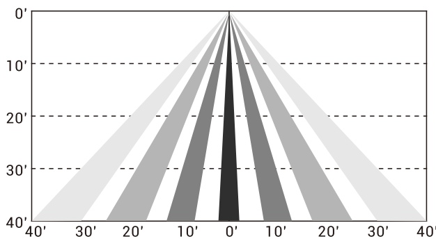
HBL1 Coverage Side View
