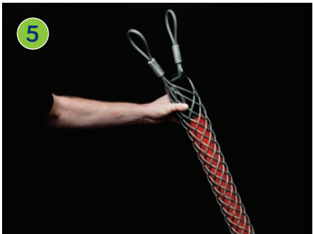
The grip then needs to be pushed along so that all the lattice is in contact with the conductor.
