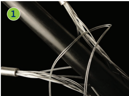
Start the lacing from the 'eye' end or anchoring end of the cable grip.
