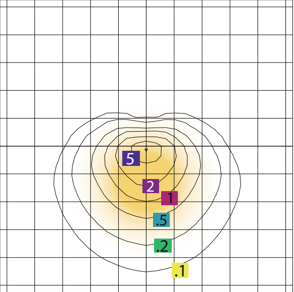
OWP300-28W Mounting Height=10.00 FT
