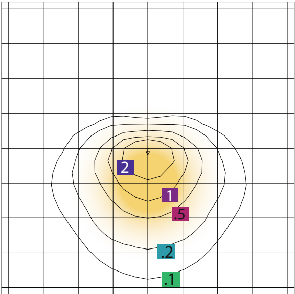
OWP200-15W Mounting Height=10.00 FT
