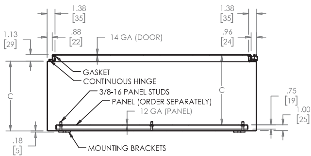
SECTION Z-Z
