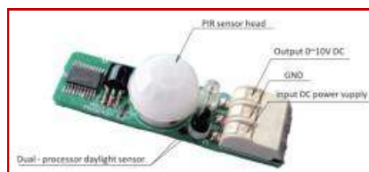
PIR Sensor
