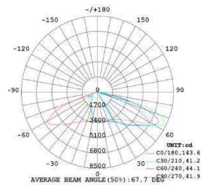
TK-SAL4-100W-T4-40K
