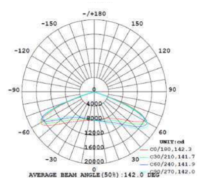
TK-SAL4-300W-T5-40K
