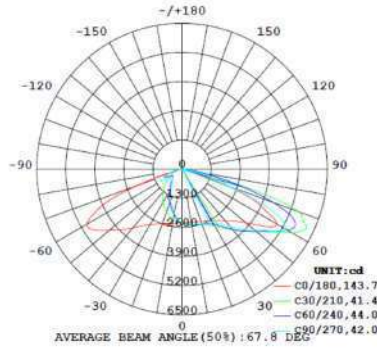
TK-SAL4-75W-T4-50K
