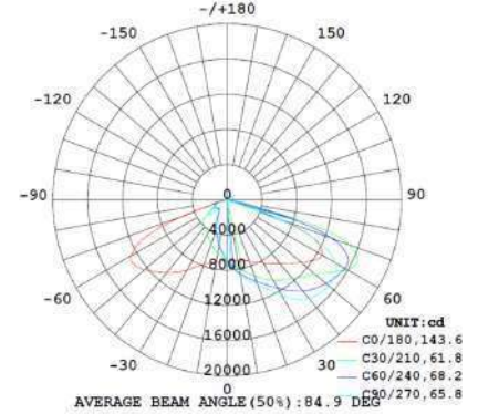
TK-SAL4-230W-T4-40K
