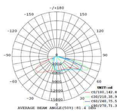
TK-SAL4-145W-T4-40K
