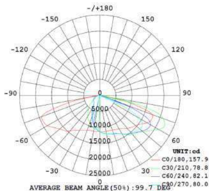
TK-SAL4-300W-T3-40K
