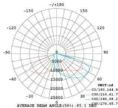
TK-SAL4-300W-T4-50K
