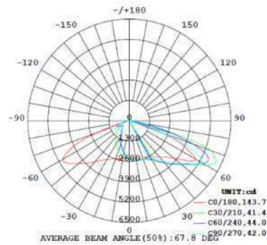
TK-SAL4-200W-T4-50K
