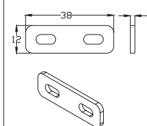
Fixing Plate
