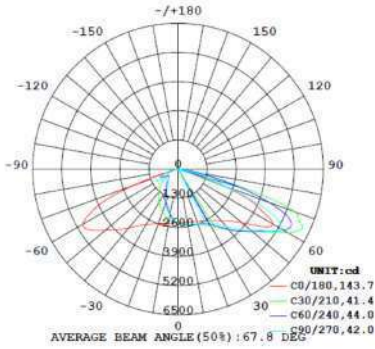
TK-SAL4-75W-T4-40K
